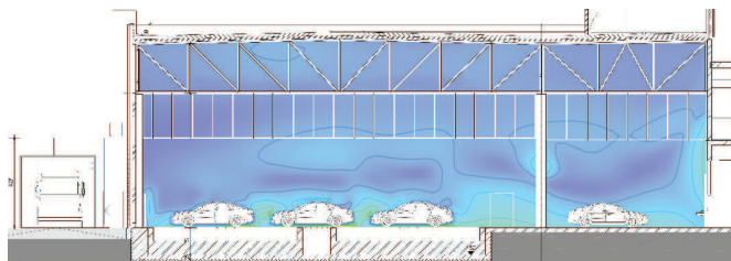
Strömungssimulation - Design Builder
